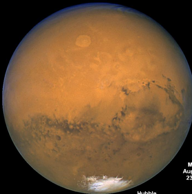
Hubble
